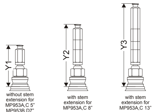
Fig. 5. Stem extensions
