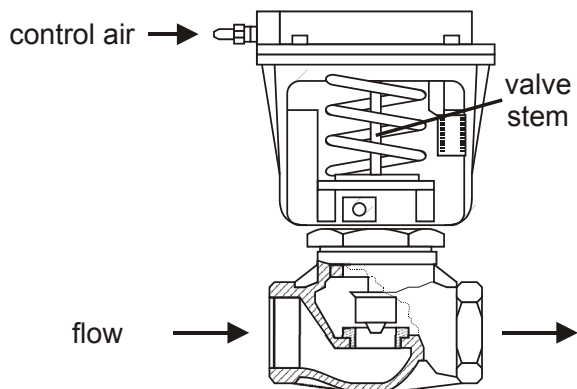
Fig. 2. Typical operation
