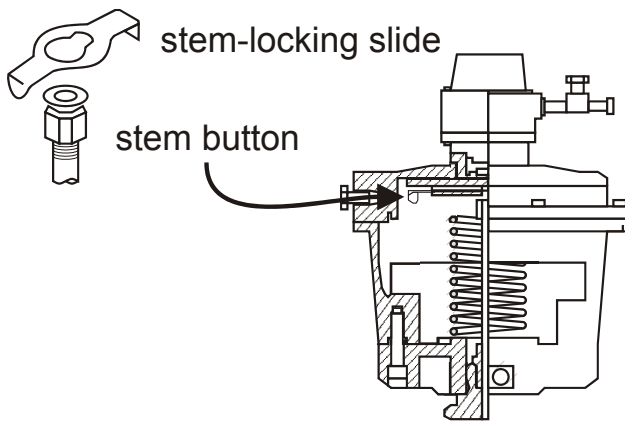
Fig. 3. Stem-locking slide
